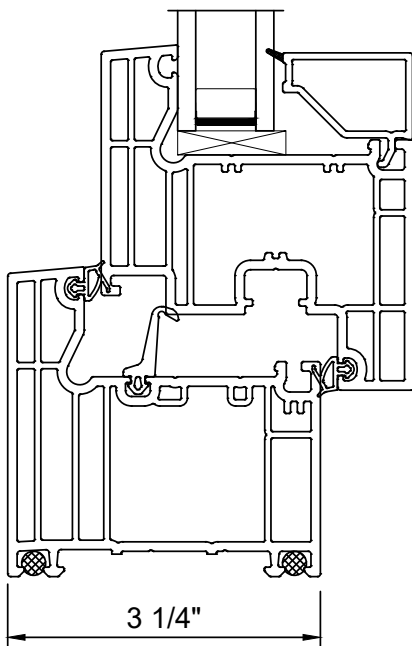
V500 Inswing
