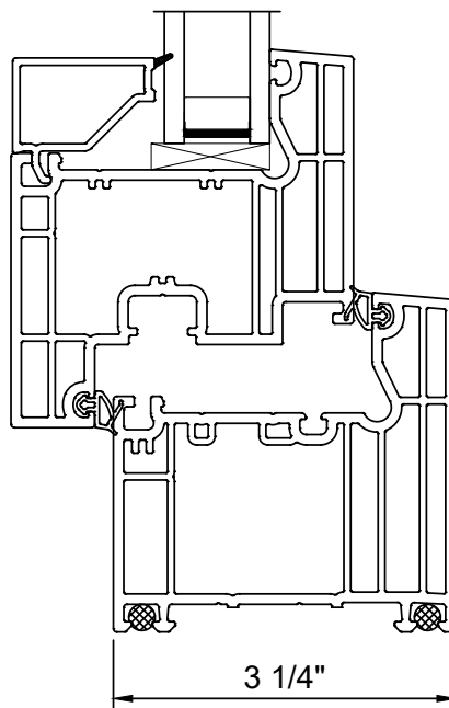
V600 Outswing
